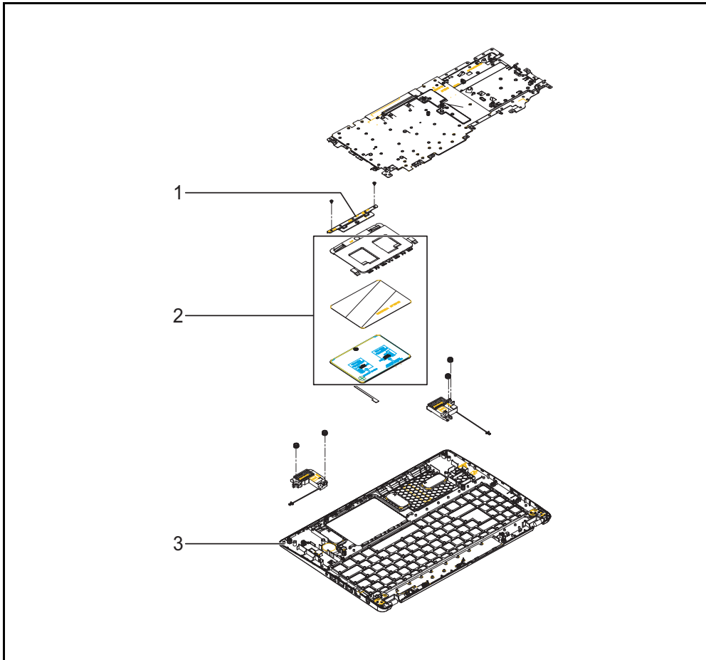
Figure 6-2. Upper Cover Assembly Exploded Diagram
