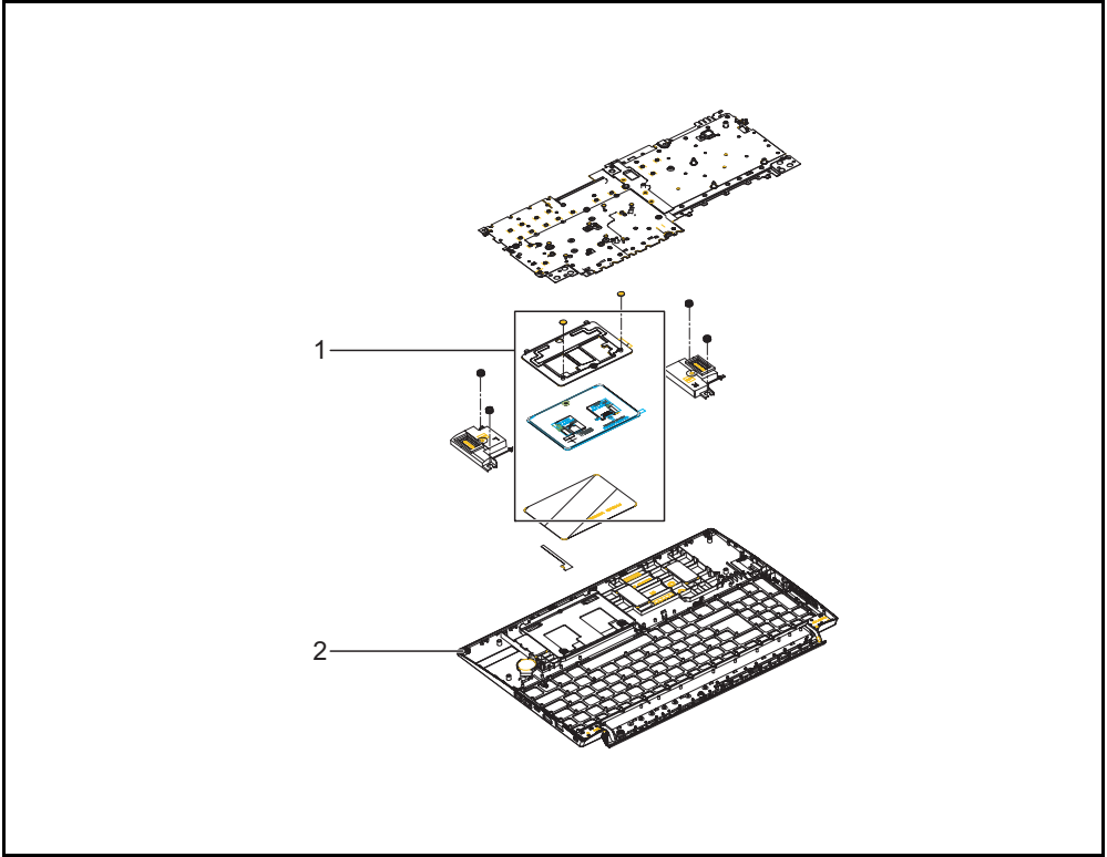
Figure 6-2. Upper Case Assembly Exploded Diagram
