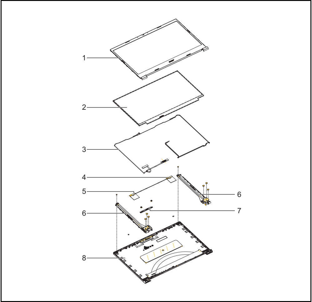
Figure 6-3. LCD Assembly Exploded Diagram Table 6-3. LCD Assembly Exploded Diagram
