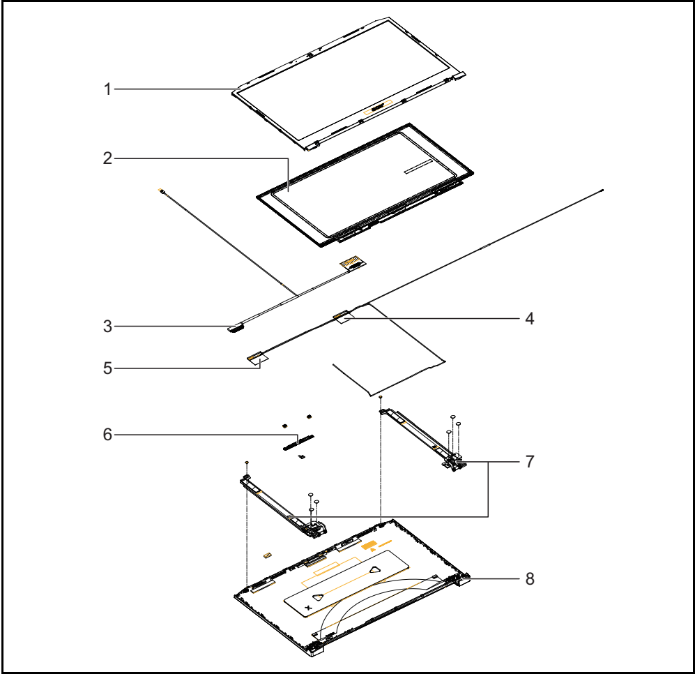
Figure 6-4. LCD Assembly Exploded Diagram Table 6-3. LCD Assembly Exploded Diagram
