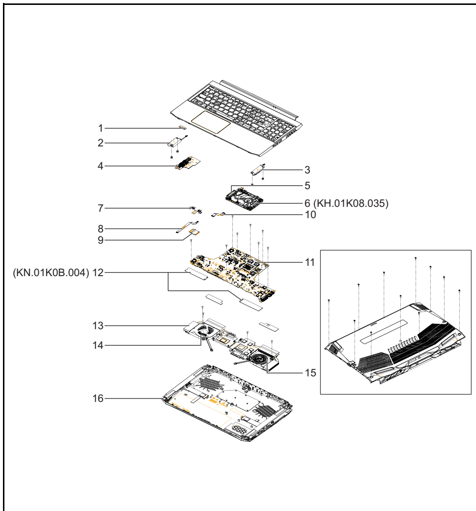
Figure 6-1. Main Assembly Exploded Diagram (N18P-G61/GN20-P0/P1)
