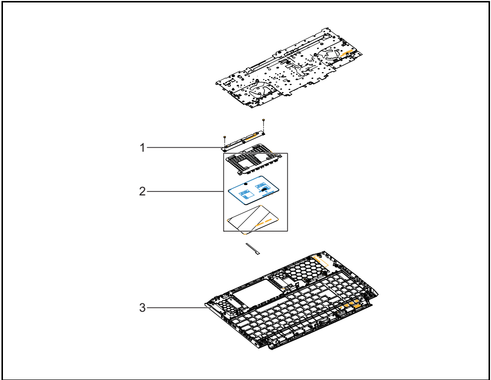
Figure 6-3. Upper Case Assembly Exploded Diagram
