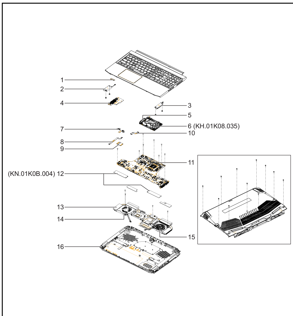
Figure 6-2. Main Assembly Exploded Diagram (GN20-E3/E5/E7)
