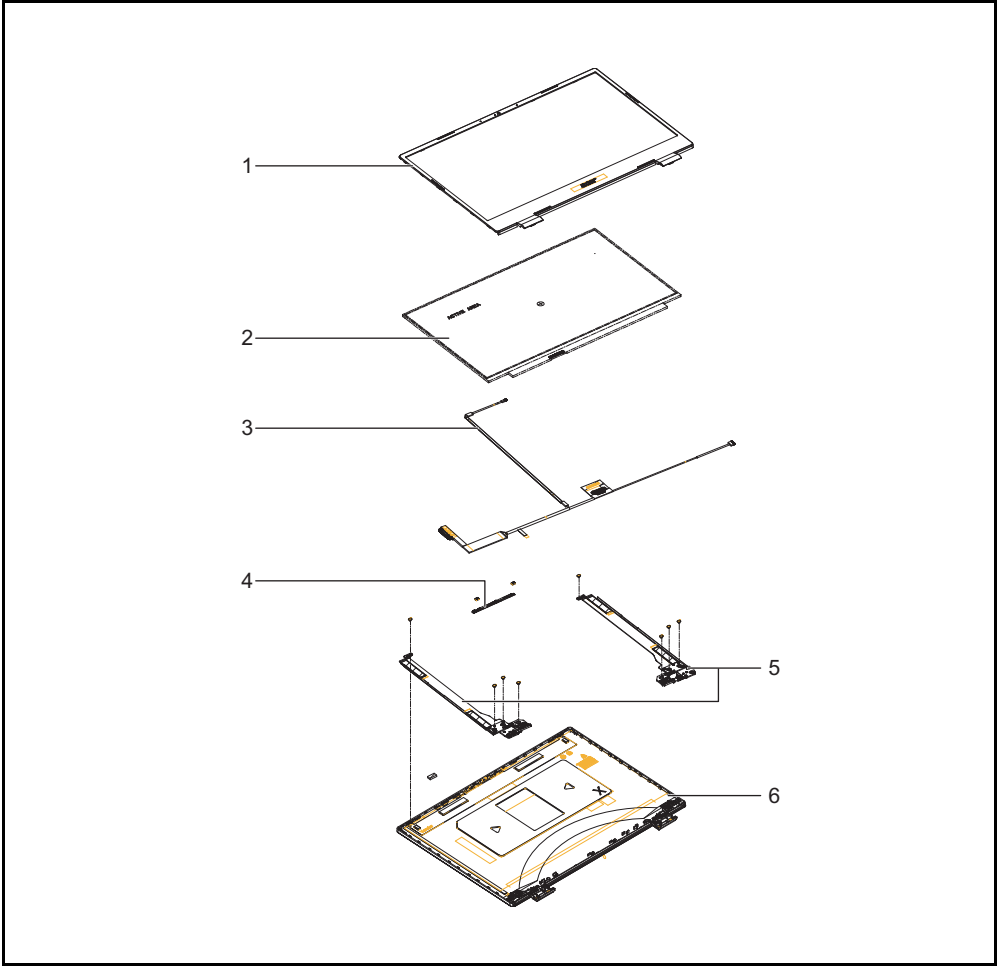
Figure 6-3. LCD Assembly Exploded Diagram
