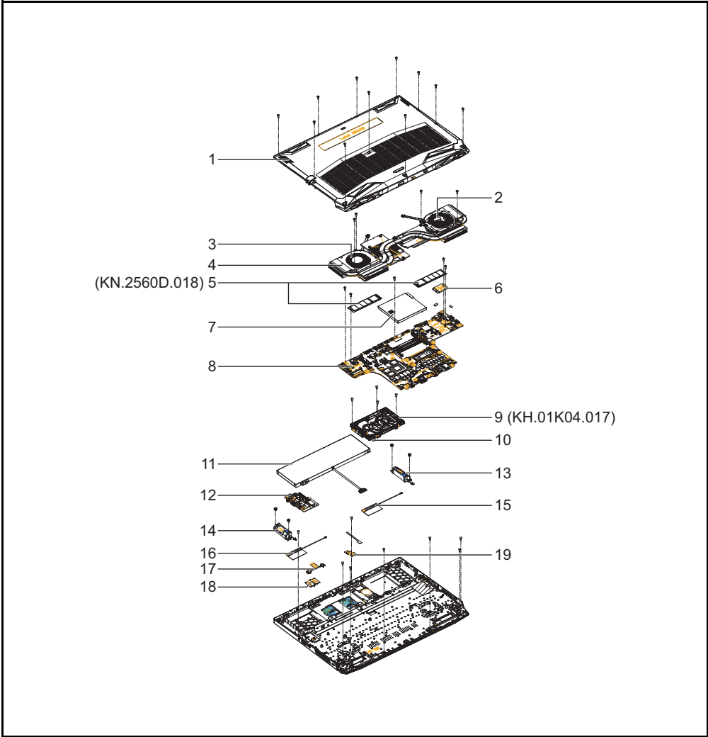
Figure 6-1. Main Assembly Exploded Diagram
