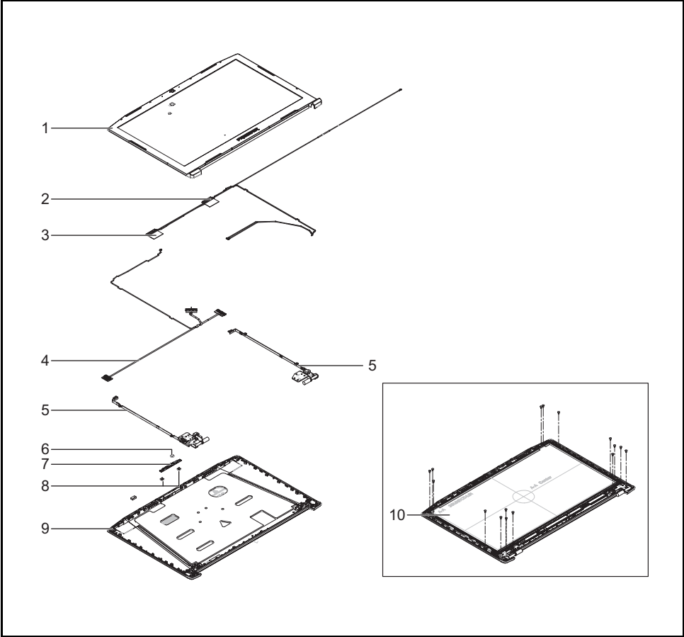
Figure 6-3. LCD Assembly Exploded Diagram
