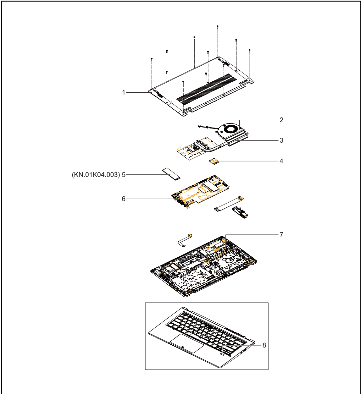
Figure 6-1. Main Assembly Exploded Diagram
