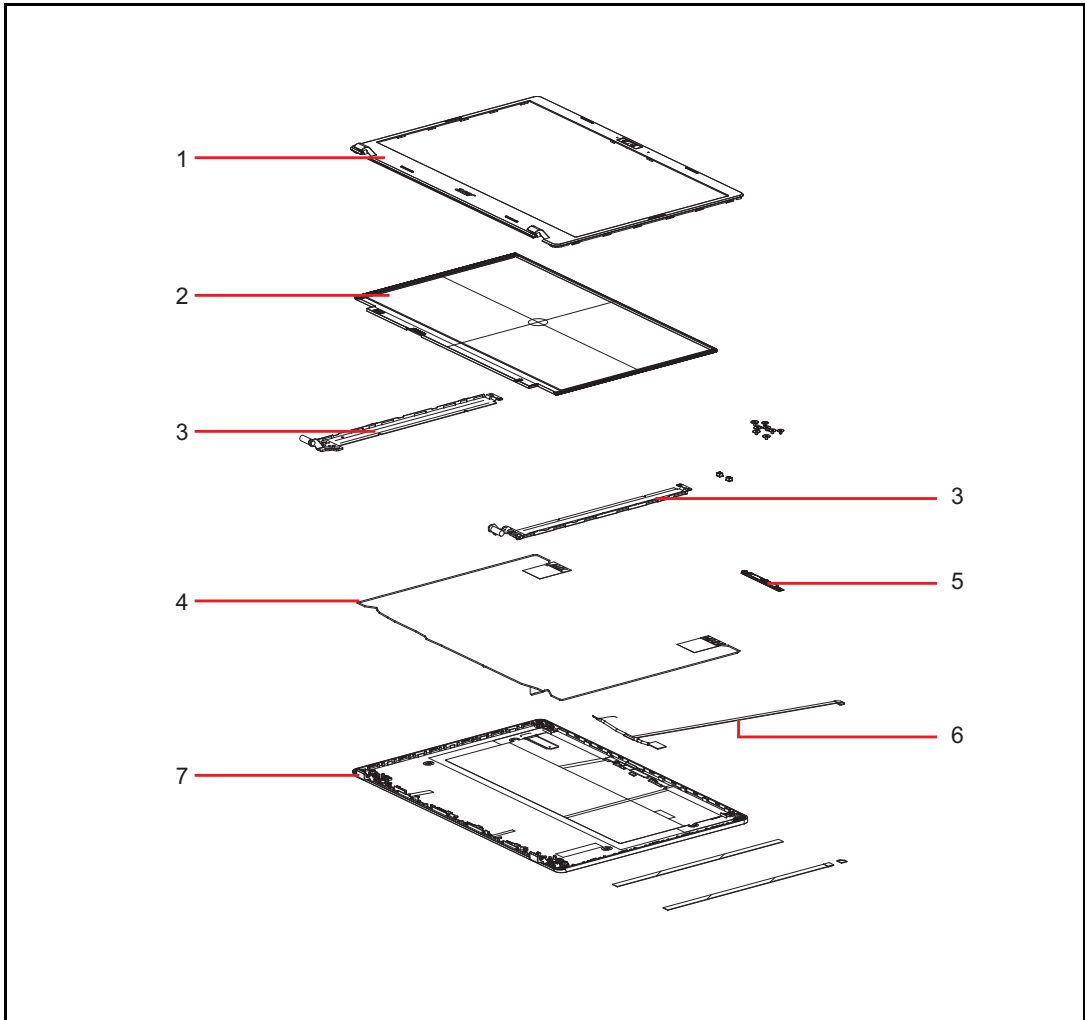
Figure 6-2. LCD Assembly Exploded Diagram
